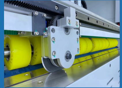
Horizontal Cutting Blade
